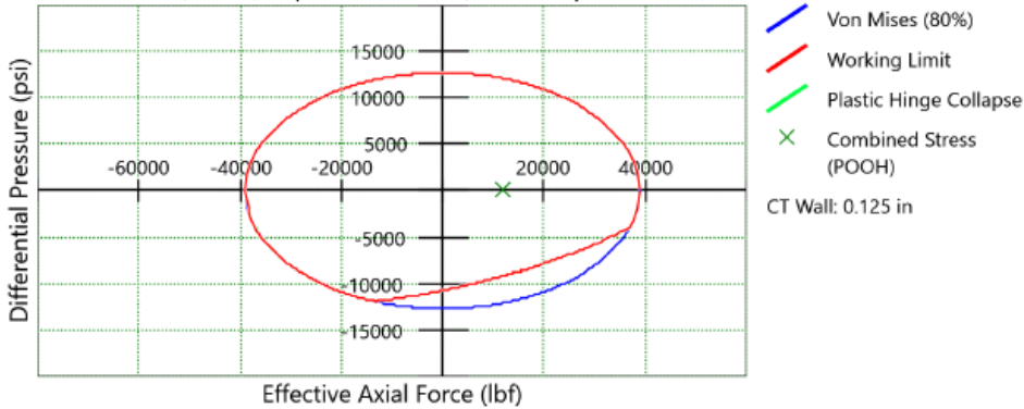
CT Limits (POOH) at position: 410 ft (at Run Depth=9384 ft)
