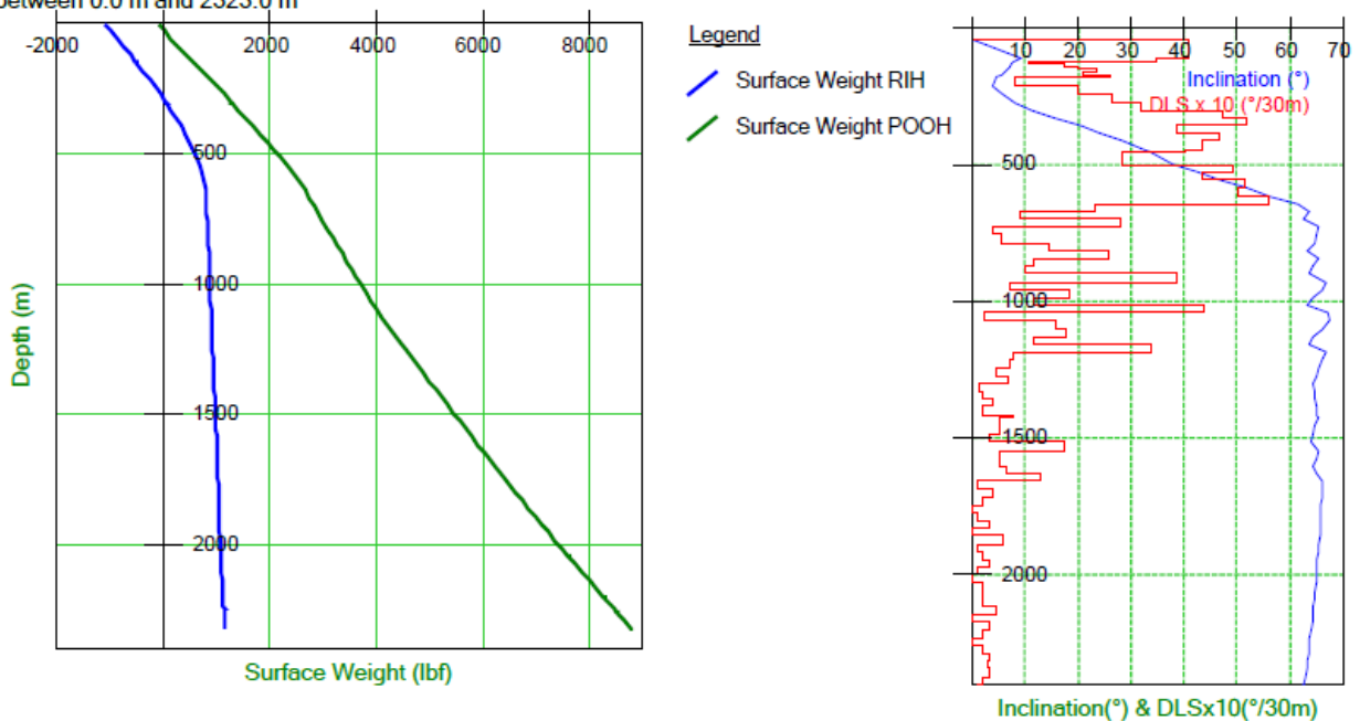
RIH and POOH between 0.0 m and 2323.0 m
