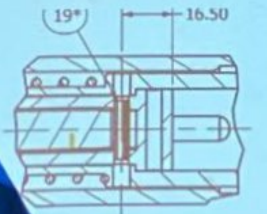
DETAIL A & PIN ON ASSEMBLY 1/16" SLOTTED SPRING PIN
