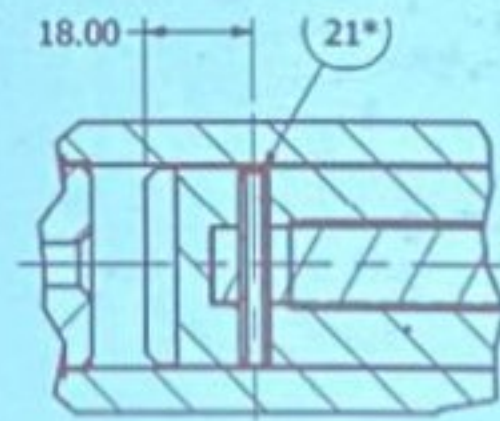
DETAIL B DRILL & PIN ON ASSEMBLY TO SUIT 3/16" SLOTTED SPRING PIN
