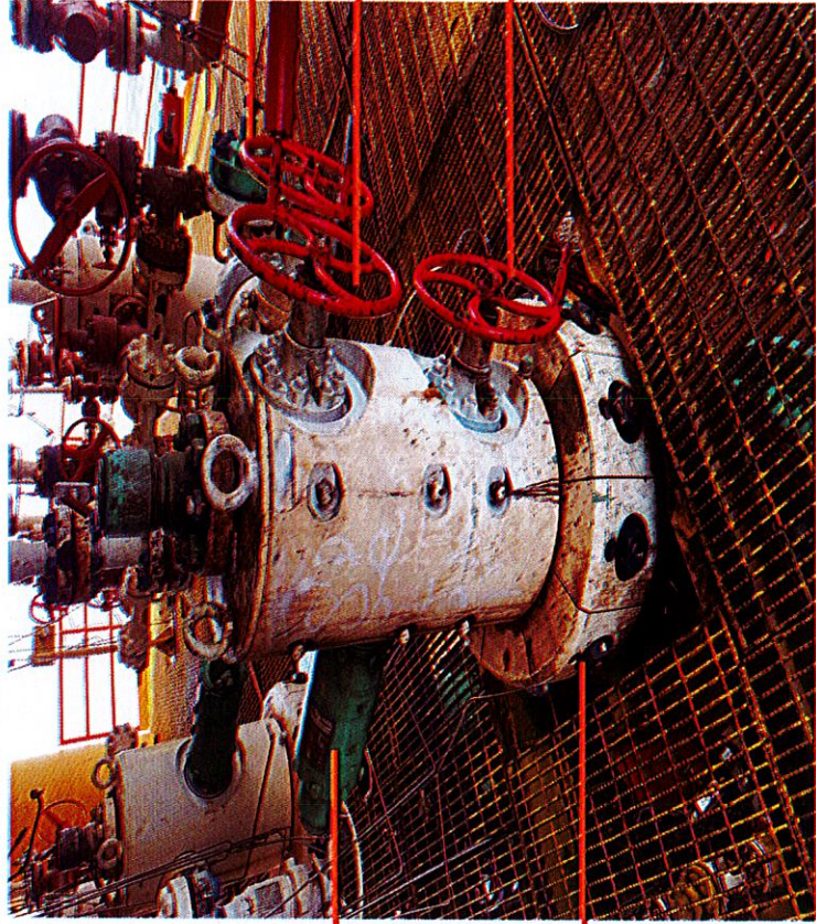
Figure 9: Wellhead/Xmas Tree configurations
