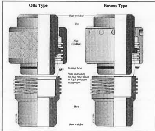
Otis Type Quick Union Dimensions
