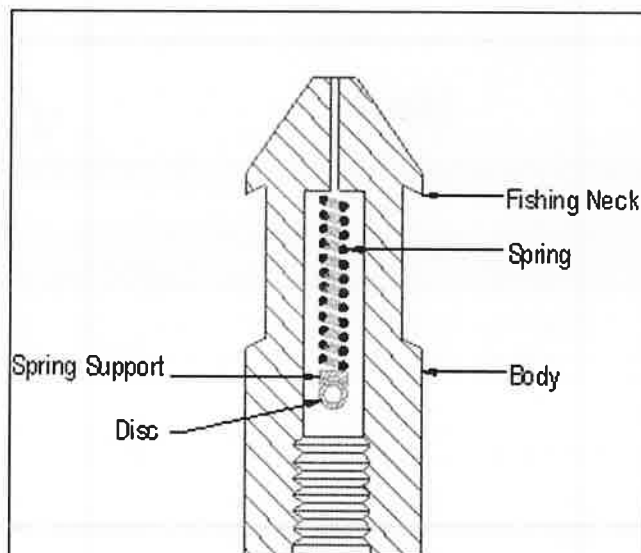
Fig 3.1-3, Conventional Type
