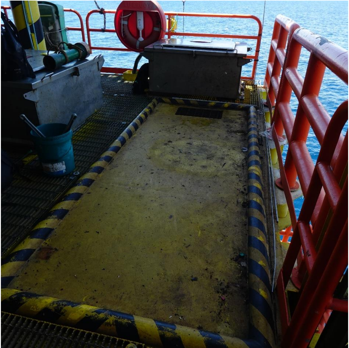
Fig: Loading Bay on Cellar Deck, In Front of Control Room. Usable Area 12 ft x 4 ft.
