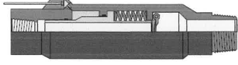
Flapper closed
